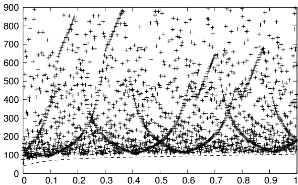
Figure 5. A scatterplot of the relation of p_1 and \mu
